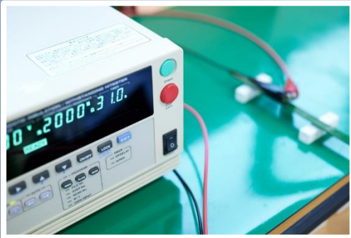
Withstanding Voltage Test
