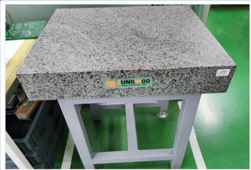
Bow and Twist Inspection
